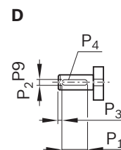
For sensor
