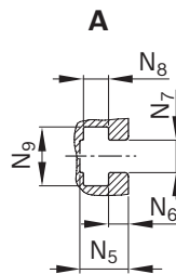
For clamping fixtures
