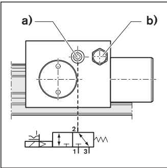
Circuit type 1) for standard air port
