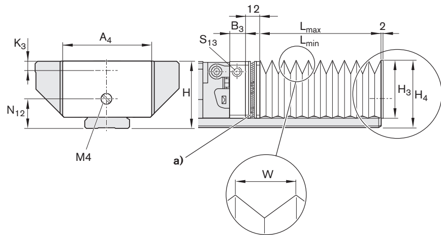
Heat-resistant bellows 2) (Note the overall height)
