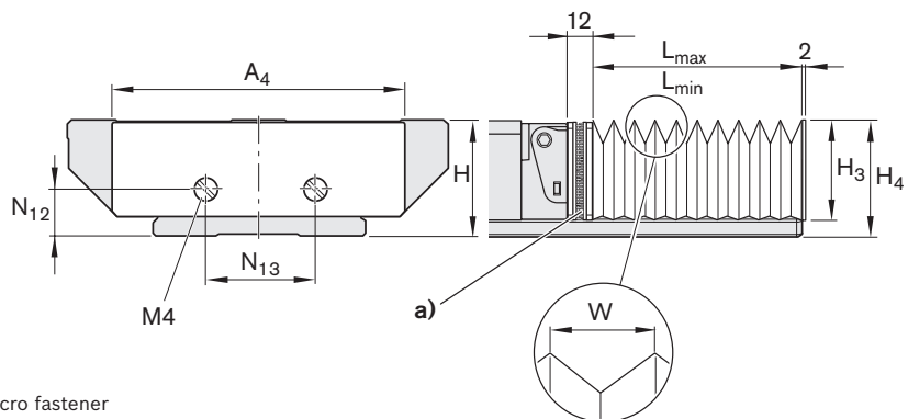
Bellows, wide
